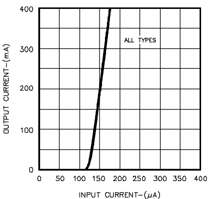
FIGURE 3. OUTPUT CURRENT VS. INPUT CURRENT
