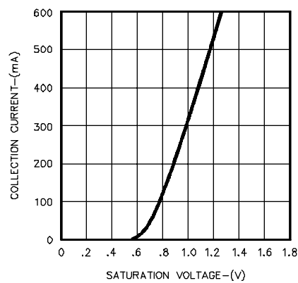
FIGURE 1. OUTPUT CHARACTERISTICS
