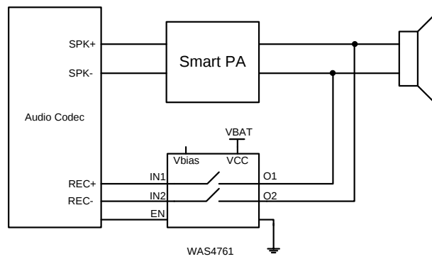
2 in 1 Speaker applications with smart PA and none cap-less receiver output
