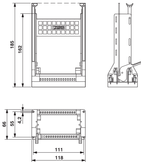
Dimensional drawing
