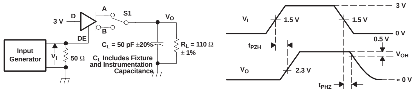
Figure 10. Driver High-Level Enable and Disable Time Test Circuit and Voltage Waveforms
