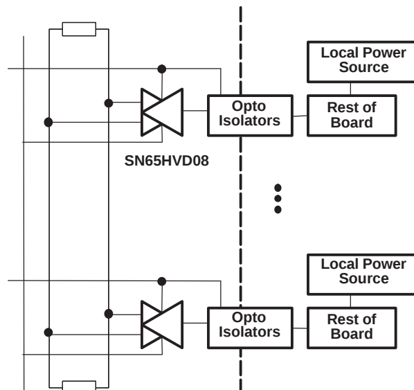
Figure 19. Distribution of Isolated Power
