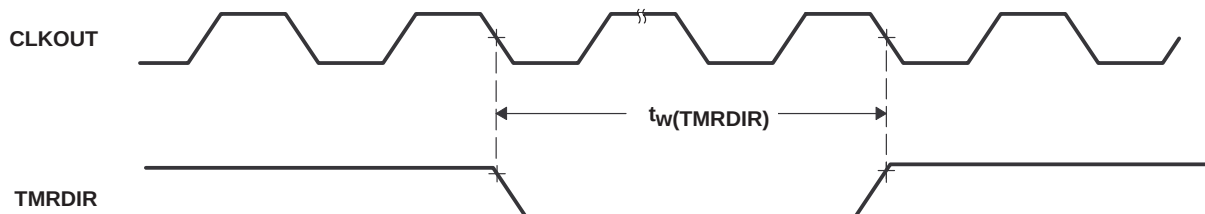
Figure 25. Capture/TMRDIR Timing
