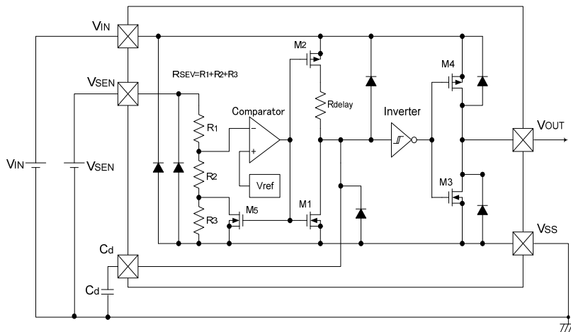
Figure 1: Typical application circuit example
