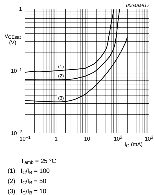
Fig 9. TR1 (NPN): Collector-emitter saturation voltage as a function of collector current; typical values
