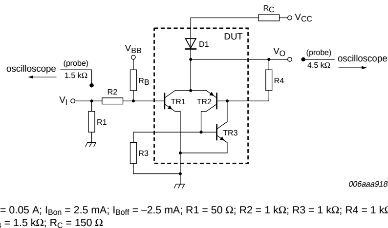
Fig 10. Test circuit for switching times per TR1
