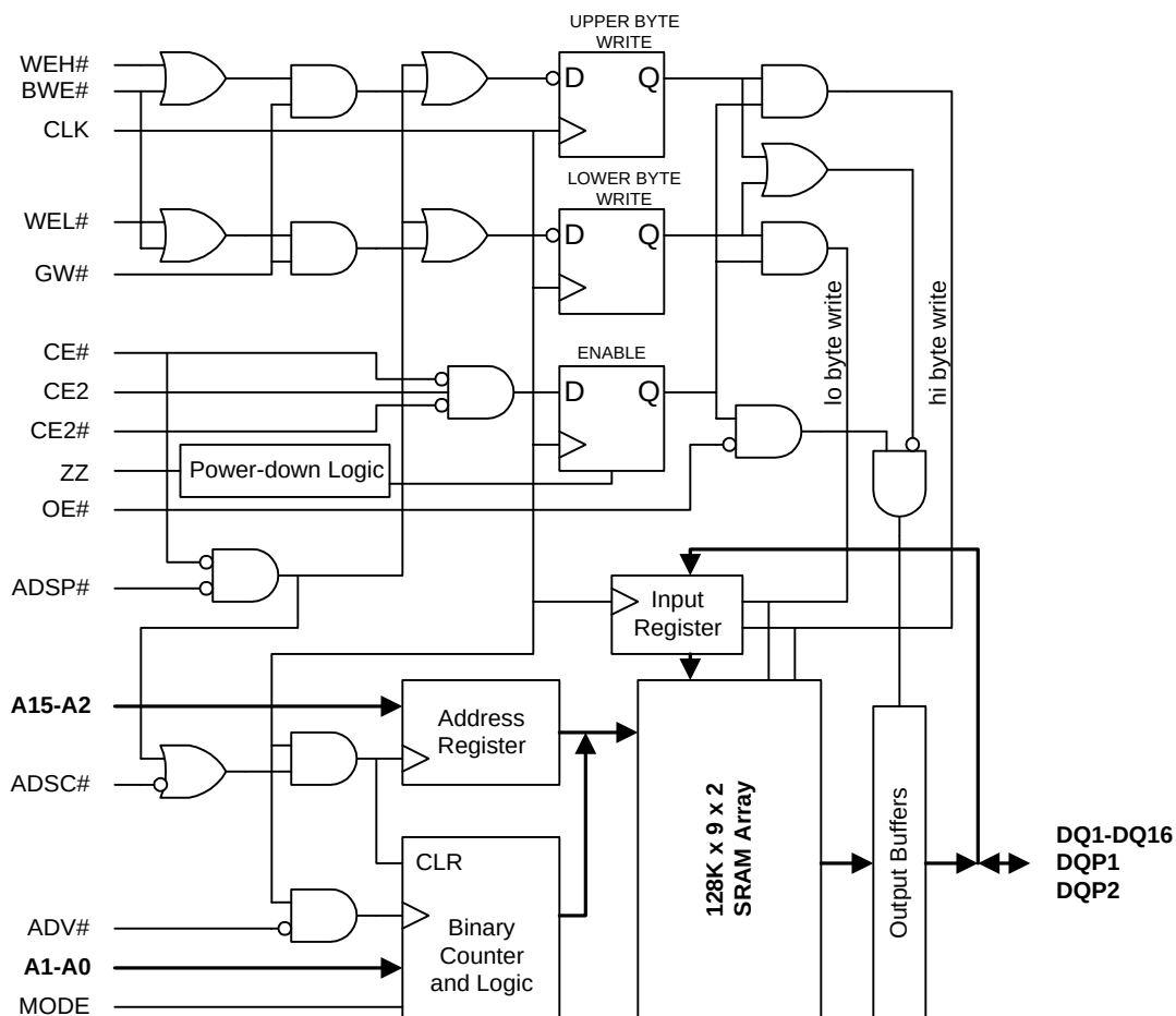
Functional Block Diagram—64Kx18 [1]
