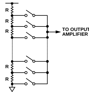
Figure 31. Resistor String
