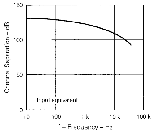
CHANNEL SEPARATION
