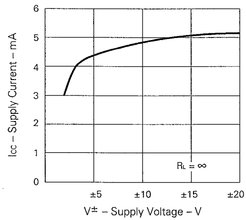
SUPPLY CURRENT
