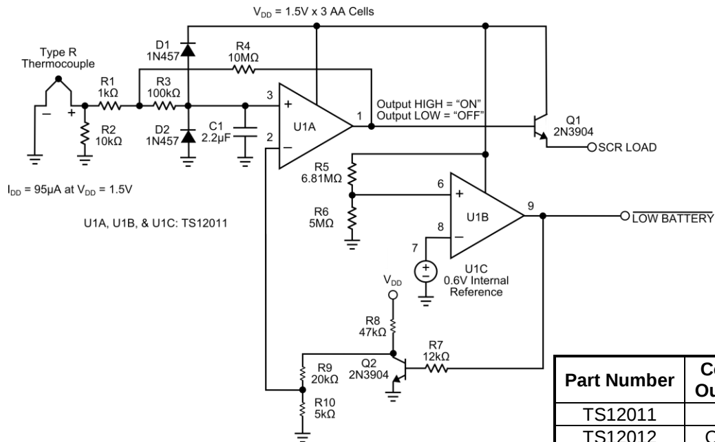
Pilot Light Flame Detector with Low-Battery Lockout Circuit
