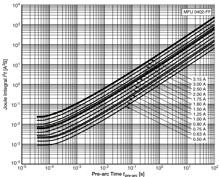
Typical I^2 t vs. t_{\text{pre-arc}} characteristic of MFU 0402 (1)
