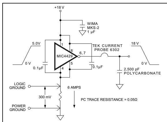
FIGURE 4-2: Switching Time Degradation Due to Negative Feedback.
