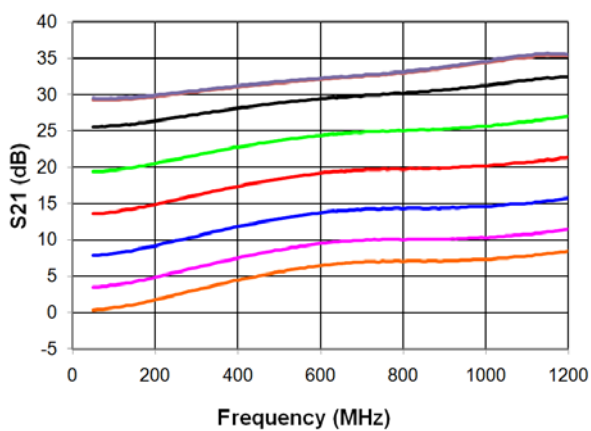
Receiver Gain vs. Frequency to 1.2 GHz
