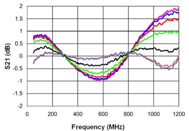
Gain Flatness Deviation From Best Fit Line
