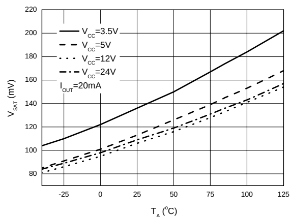
Figure 12. V_{SAT} vs. T_A
