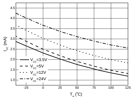
Figure 10. I_{CC} vs. T_A
