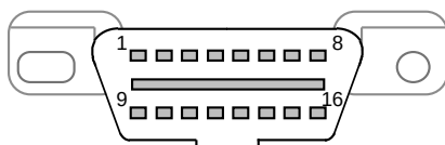
Figure 3. Vehicle Connector
