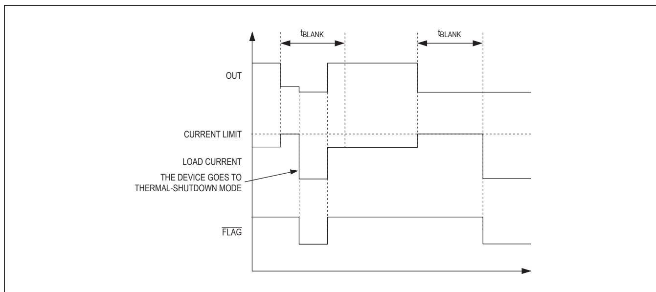
Figure 2. Latchoff Fault Diagram
