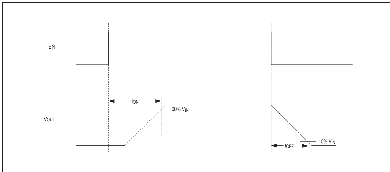
Figure 1. Timing Diagram for Measuring Turn-On Time and Turn-Off Time
