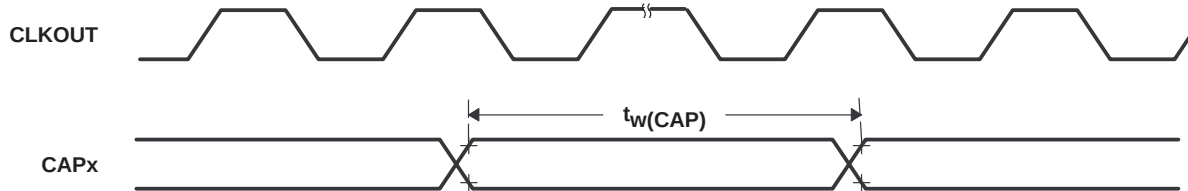
Figure 30. Capture Input and QEP Timing
