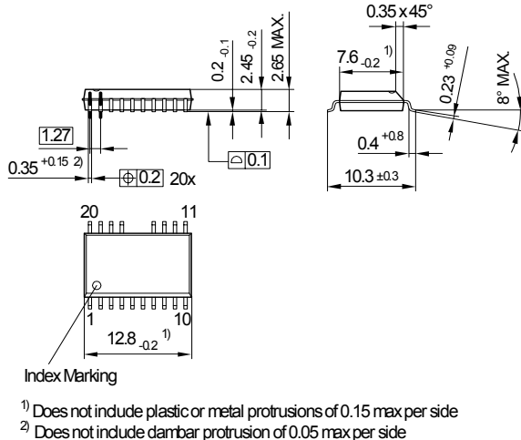
Figure 20 Package dimensions and mechanical data (Dimensions in mm).
