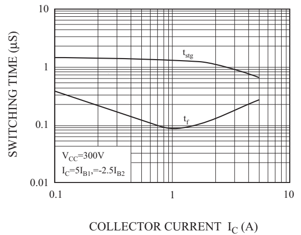
Fig 6. SWITCHING CHARACTERISTIC
