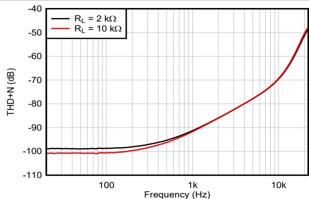
Figure 6-12. THD+N Ratio vs Frequency, G = 1 G = 1 , f = 1\text{ kHz} , BW = 80\text{ kHz} , V_{OUT} = 10\text{ V}_{PP} , R_L connected to V_-
