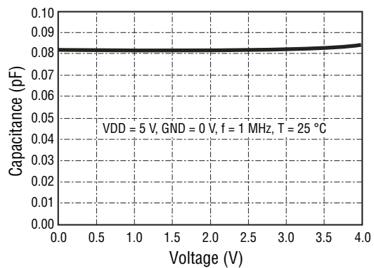
Typical Variation of C_{IO\text{-to-}IO} vs. V_{IN}
