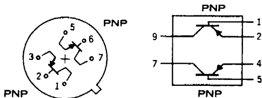
PIN CONNECTIONS (BOTTOM VIEW)
