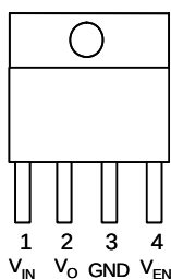
TO-220F-4
