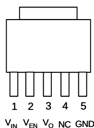
TO-252-5
