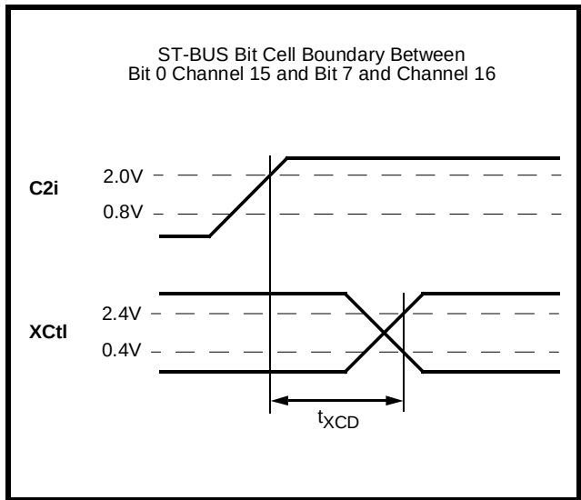
Figure 23 - XCTL Timing
