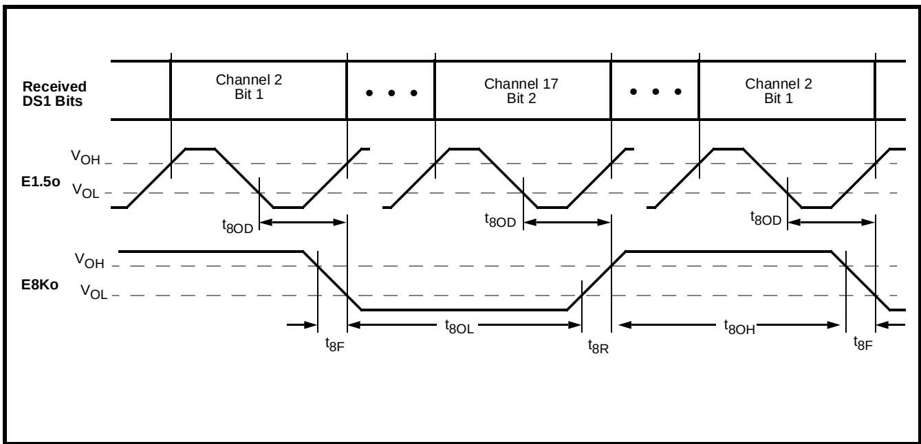
Figure 25 - E8Ko Timing
