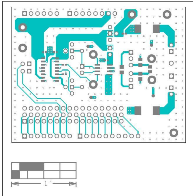
MAX33046E EV Kit PCB Layout—Top Layout
