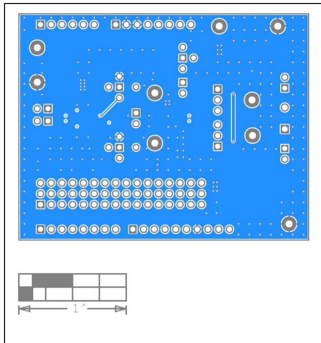
MAX33046E EV Kit PCB Layout—Bottom Layout
