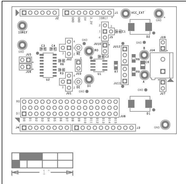
MAX33046E EV Kit Component Placement Guide—Top Silkscreen
