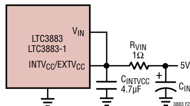
Figure 23. Setup for a 5V Input
