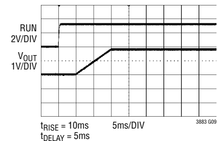
Soft-Start Ramp
