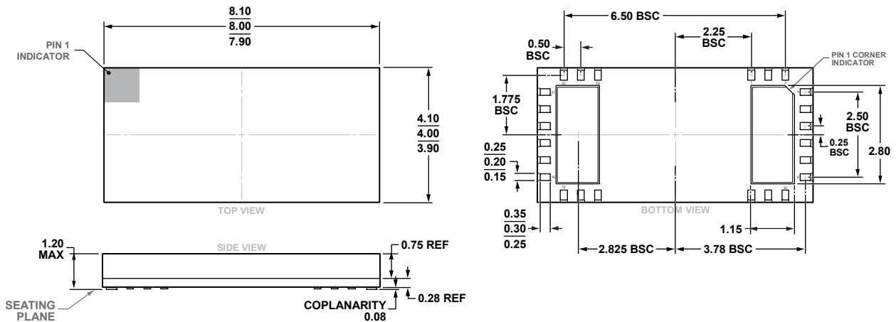
Figure 29. 24-Terminal Land Grid Array [LGA]
