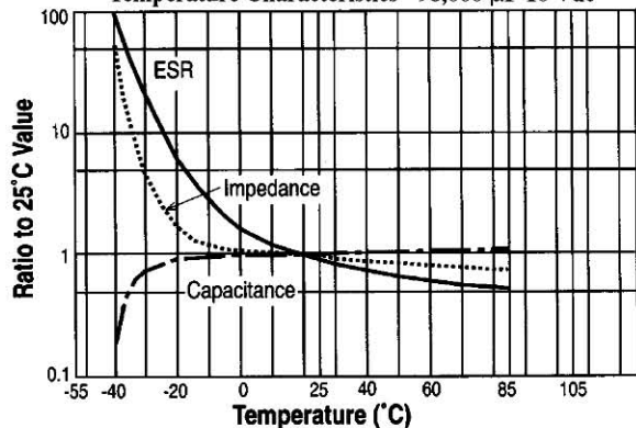
Temperature Characteristics - 98,000 \mu F 10 Vdc
