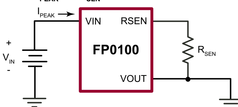
Figure 2. Test Circuit for I_{PEAK} vs R_{SEN}
