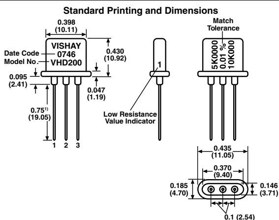
FIGURE 3 - VHD200 AND VHD144 STANDARD PRINTING AND DIMENSIONS in inches (millimeters)
