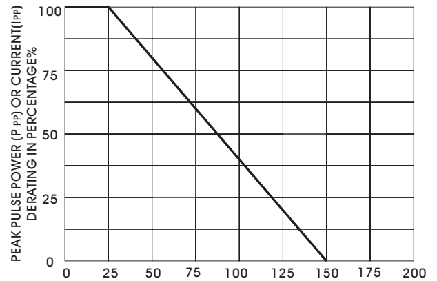
FIGURE 2 DERATING CURVE
