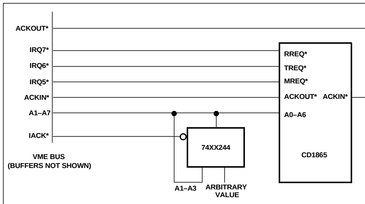
Figure 19. Incorrect VME Interface
