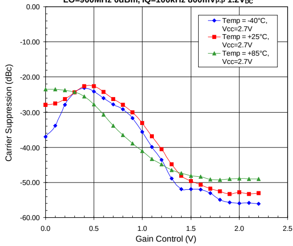
Low Band Carrier Suppression versus Gain Control V CC =2.7V, LO=0dBm, IQ=100kHz 800mV P-P 1.2V DC
