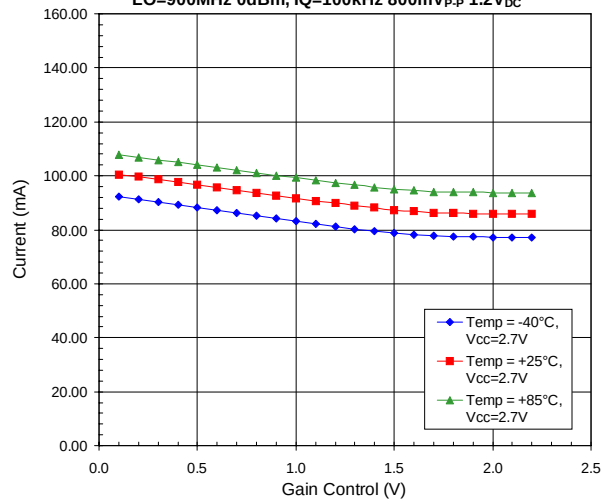
Low Band Current Consumption versus Gain Control
