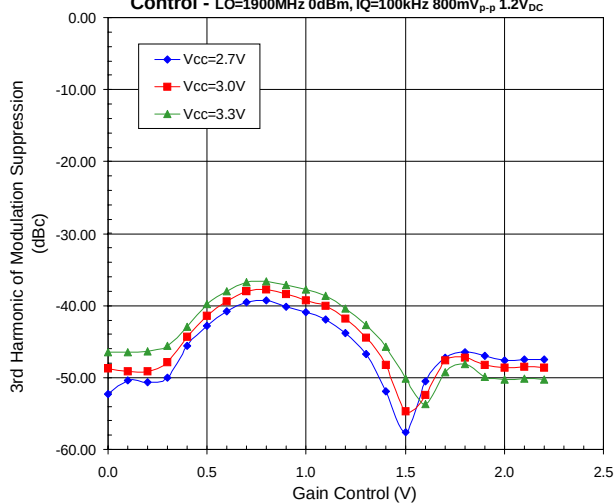
High Band Modulation's 3rd Harmonic versus Gain Control -
