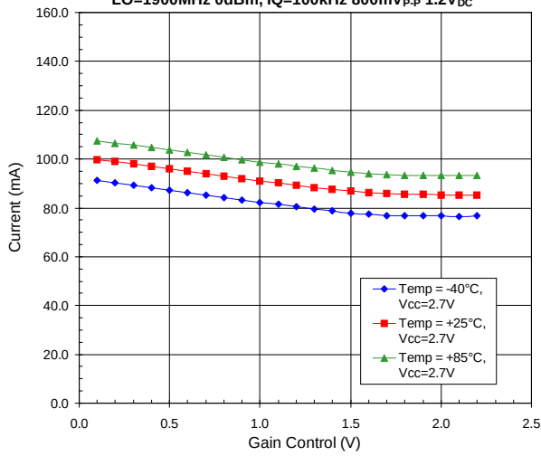
High Band Current Consumption versus Gain Control
