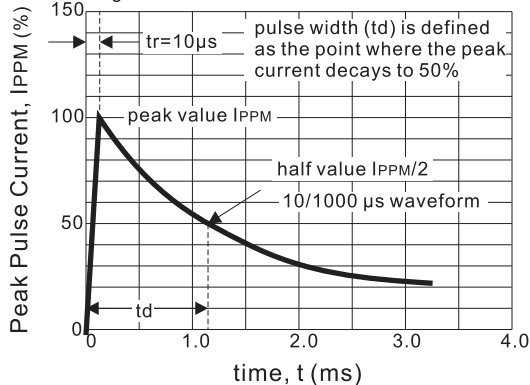
Fig.3 - Pulse Waveform
