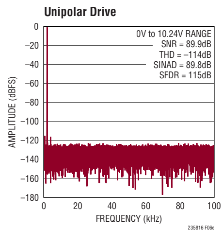
Figure 6e. IN^+ = -1\text{dBFS} 2kHz Unipolar Sine, IN^- = 0\text{V} , 32k Point FFT, f_{\text{SAMPL}} = 200\text{kps} . Circuit Shown in Figure 6a
