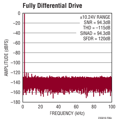
Figure 6c. IN^+/IN^- = -1\text{dBFS} 2kHz Fully Differential Sine, V_{\text{CM}} = 0\text{V} , 32k Point FFT, f_{\text{SAMPL}} = 200\text{kps} . Circuit Shown in Figure 6a
