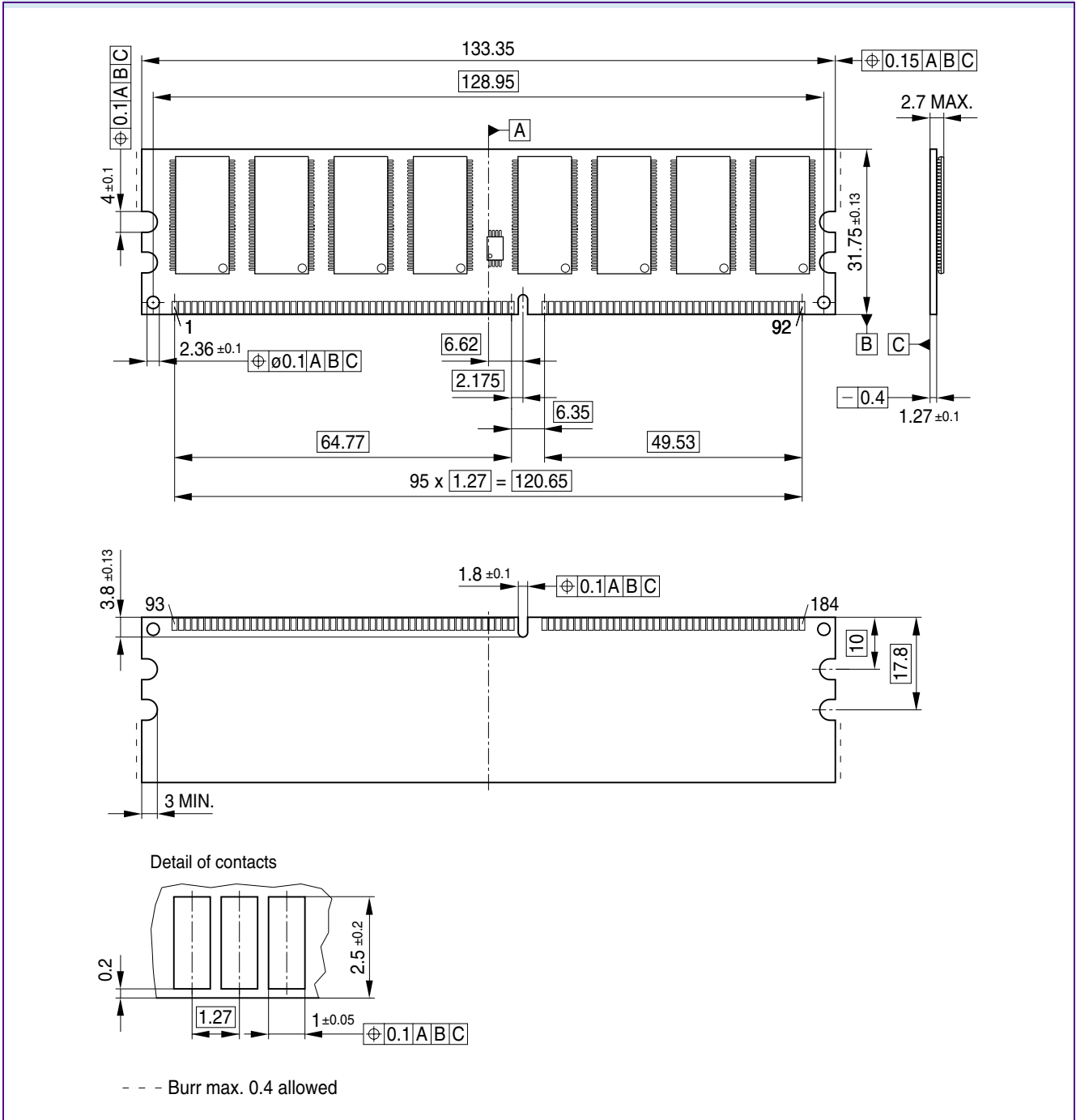
Package Outline UDIMM Raw Card A (L-DIM-184-32)
