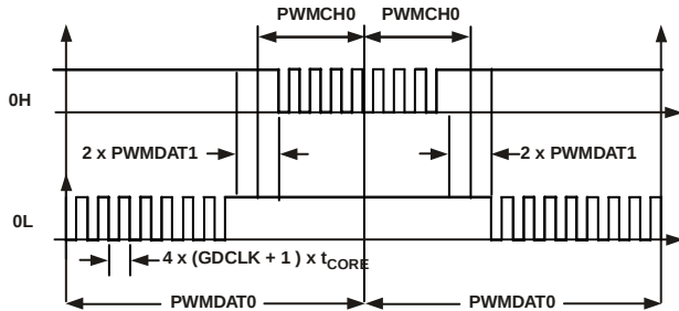
Figure 25: typical PWM signals with high frequency gate chopping enabled on both high-side and low-side switches
