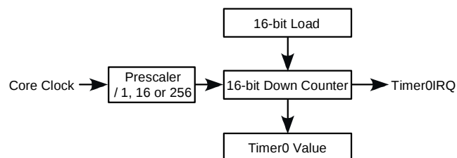
Figure 28:timer 0 block diagram
