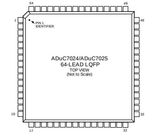
64-Lead LQFP
