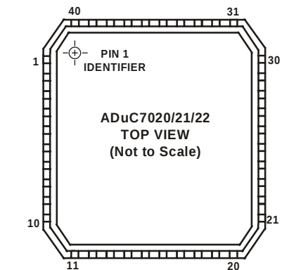
40-Lead CSP
