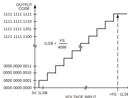
Figure 8: ADC transfer function in pseudo differential mode or single-ended mode
