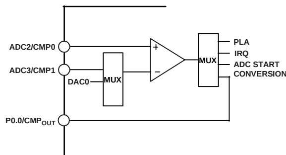
Figure 19: Comparator
