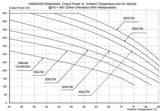
Figure 21: Output Power vs. ambient temperature and air velocity @ V_{in}=48V , V_{out}=54V (Either Orientation)
