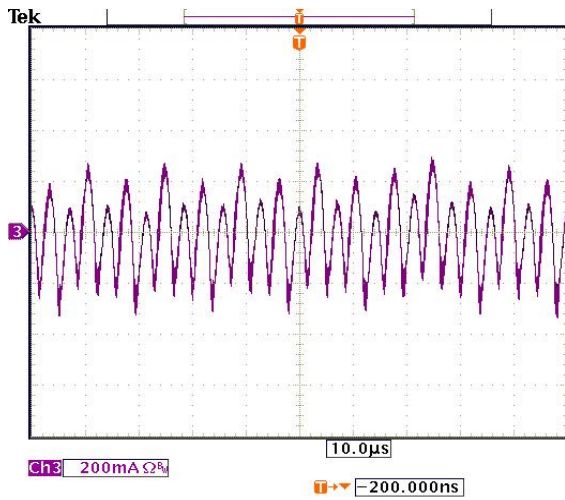
Figure 9: Input Terminal Ripple Current, i_c , at nominal input voltage and rated load current with 12\mu\text{H} source impedance and 150\mu\text{F} electrolytic capacitor (200 mA/div).
