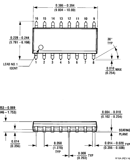
Small Outline Package (M) Order Number DS26LS32CM or DS26LS32ACM NS Package Number M16A
