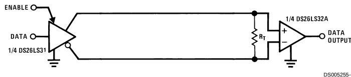
Two-Wire Balanced Interface — RS-422
