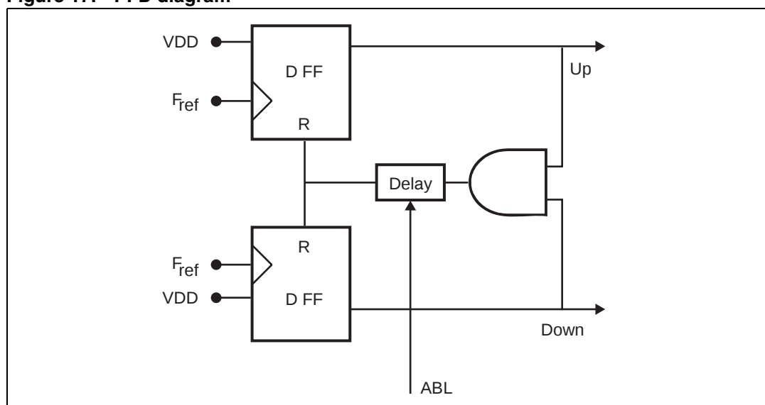
Figure 17. PFD diagram
