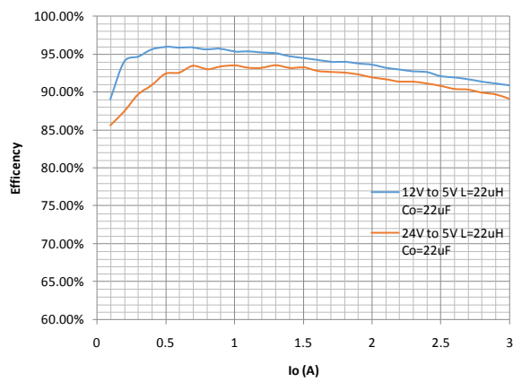
Fig. 3 Efficiency
