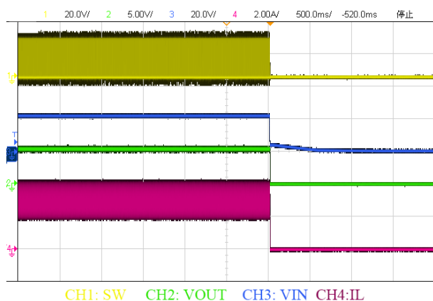
Fig. 14 Shutdown waveform, Iout = 3A
