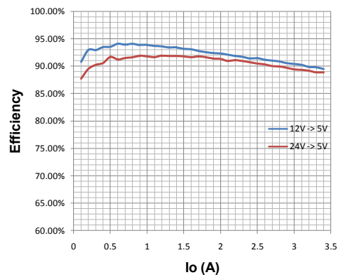
Fig. 2 Efficiency curve
