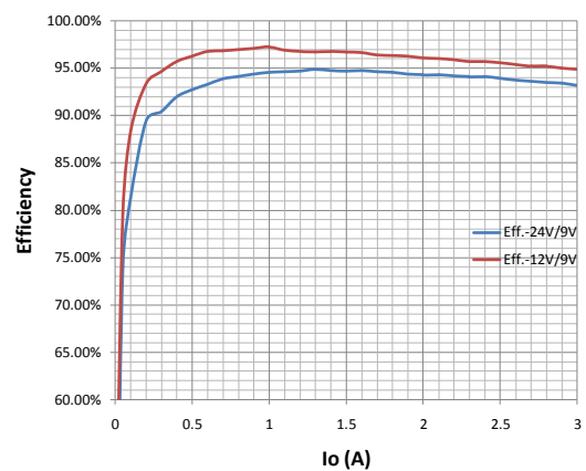
Fig. 4 Efficiency
