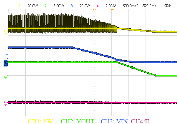
Fig. 13 Shut down waveform, Iout = 0A
