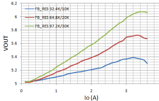
Fig. 16 line drop compensation
