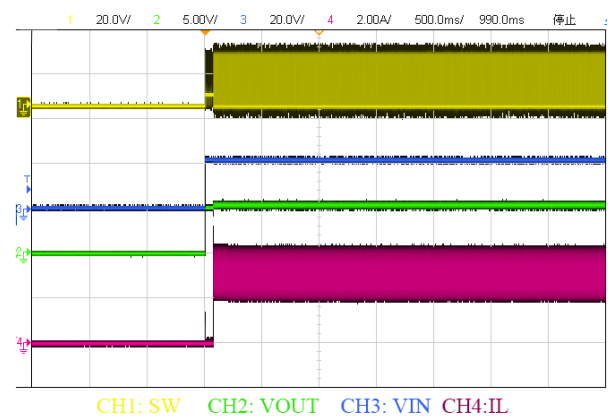
Fig. 12 Startup waveform, Iout = 3A
