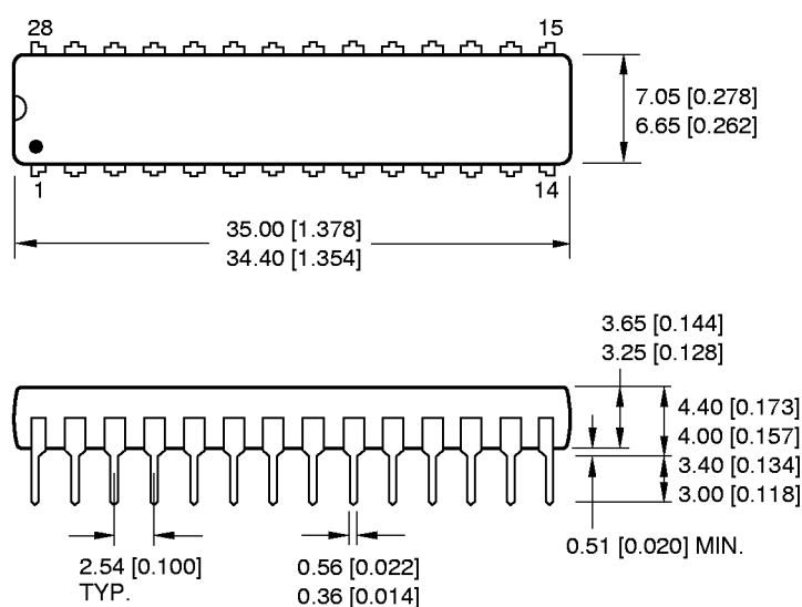
28SK-DIP (DIP028-P-0300)
