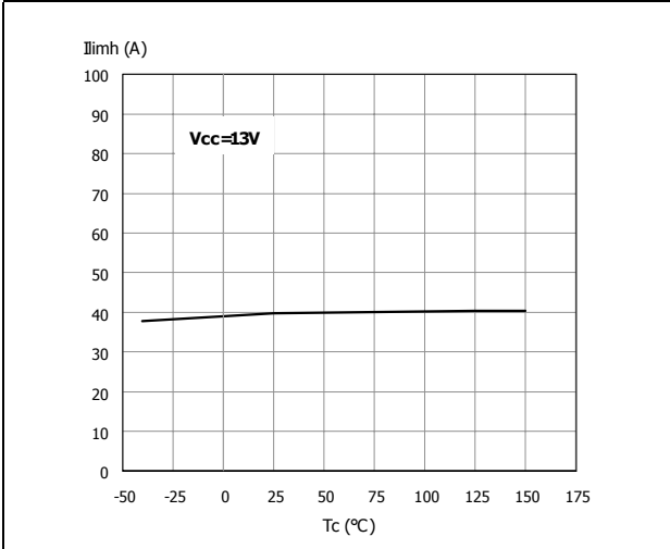
Figure 21. I_{LMH} vs. T_{case}
