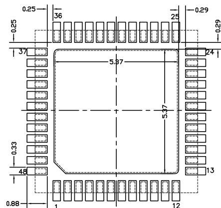
TYPICAL RECOMMENDED LAND PATTERN
