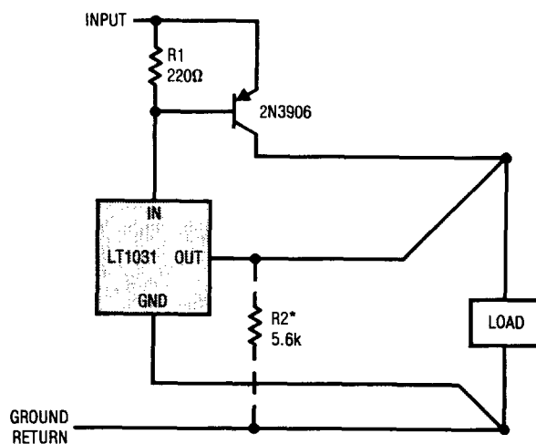
Series Mode with Boost Transistor
