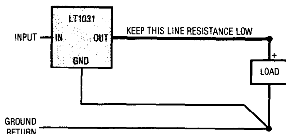
Standard Series Mode
