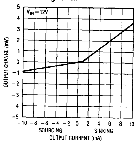
Load Regulation
