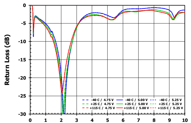
Figure 38. Output Return Loss - High Power Mode, Broadband
