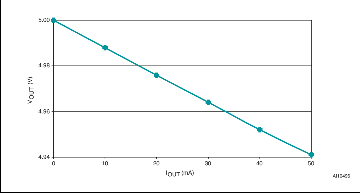
Figure 19. Output voltage vs. load current ( V_{CC} = 5\text{ V} ; T_A = 25\text{ }^\circ\text{C} )
