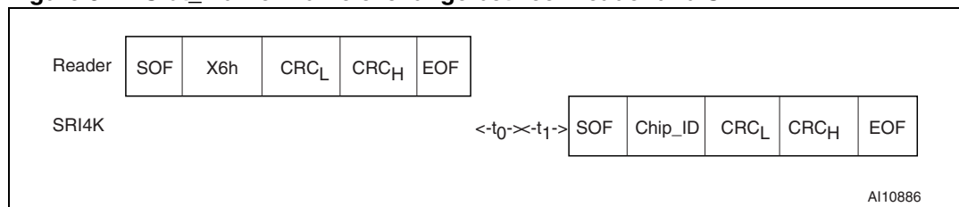
Figure 31. Slot_marker frame exchange between reader and SRI4K
