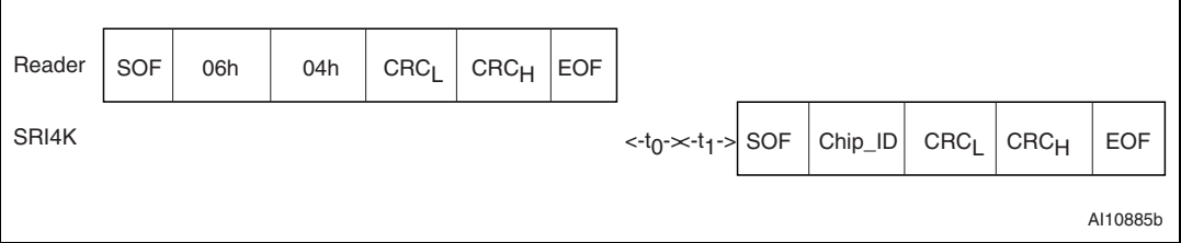
Figure 28. Pcall16 frame exchange between reader and SRI4K
