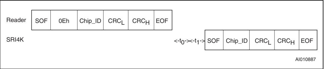
Figure 34. Select frame exchange between reader and SRI4K
