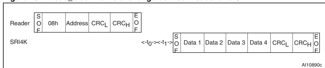
Figure 43. Read_block frame exchange between reader and SRI4K
