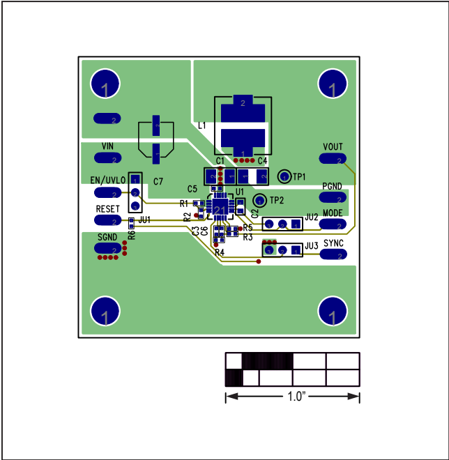
Figure 13. MAX17543 3.3V Output EV Kit Component Side PCB layout
