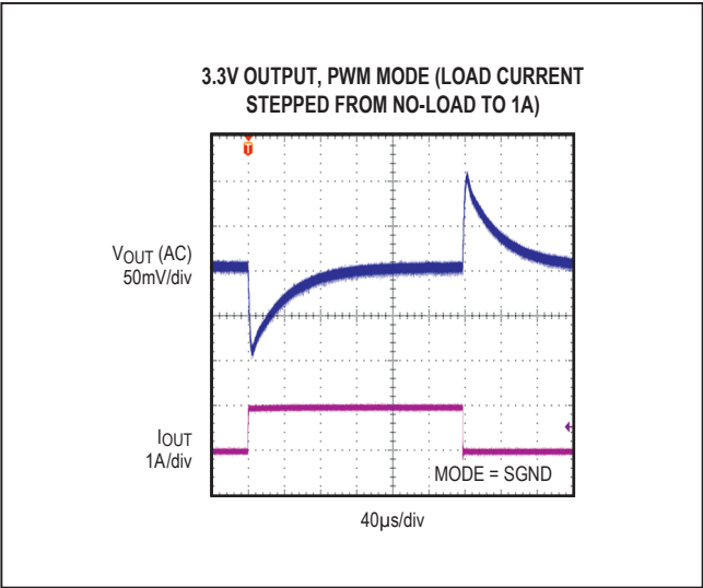
Figure 7. MAX17543 3.3V Output, No Load to 1A Load Transient (PWM Mode)
